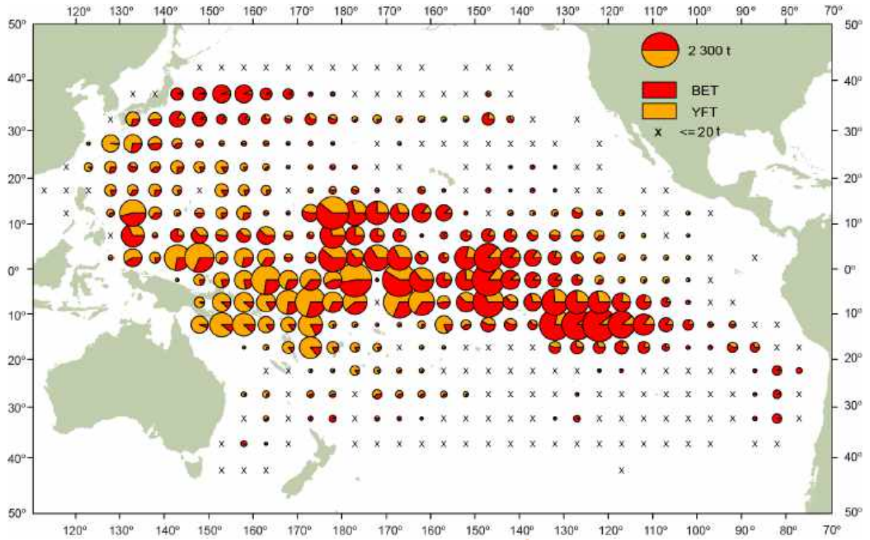
FIGURE A-4. Distributions of the average annual catches of bigeye and yellowfin tunas in the Pacific Ocean, in metric tons, by Chinese, Japanese, Korean, and Chinese Taipei longline vessels, 2016-2020. The sizes of the circles are proportional to the amounts of bigeye and yellowfin caught in those 5° by 5° areas.
