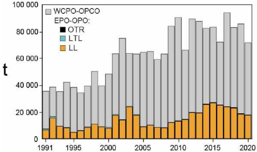
FIGURE F-1a. Retained catches of South Pacific albacore, by region. EPO catches broken down by gear: LL: longline; LTL: troll; OTR: other
