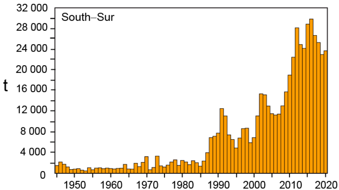
FIGURE G-4. Retained catches of swordfish in the South EPO for 1945–2020.
