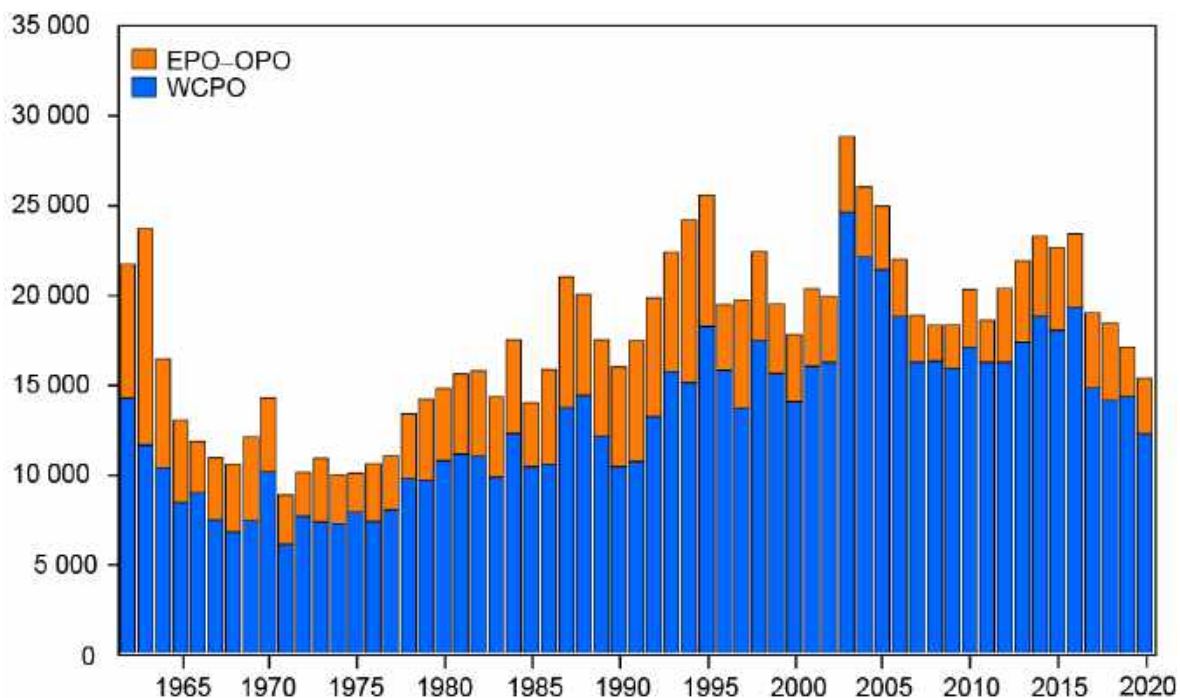
FIGURE H-1. Retained catches of blue marlin in the Pacific Ocean, by region.
